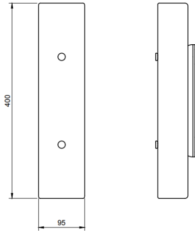
Dims: 95mm W x 400mm H x 80mm D Weight: 1kg
